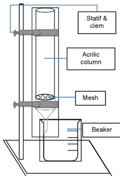
Figure 1. An illustration of filtering tube.
