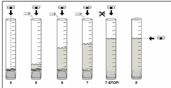
Figure 2. An illustration of processing water turbidity measurement [9].
