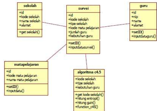
Figure 3.4 Class Diagram
