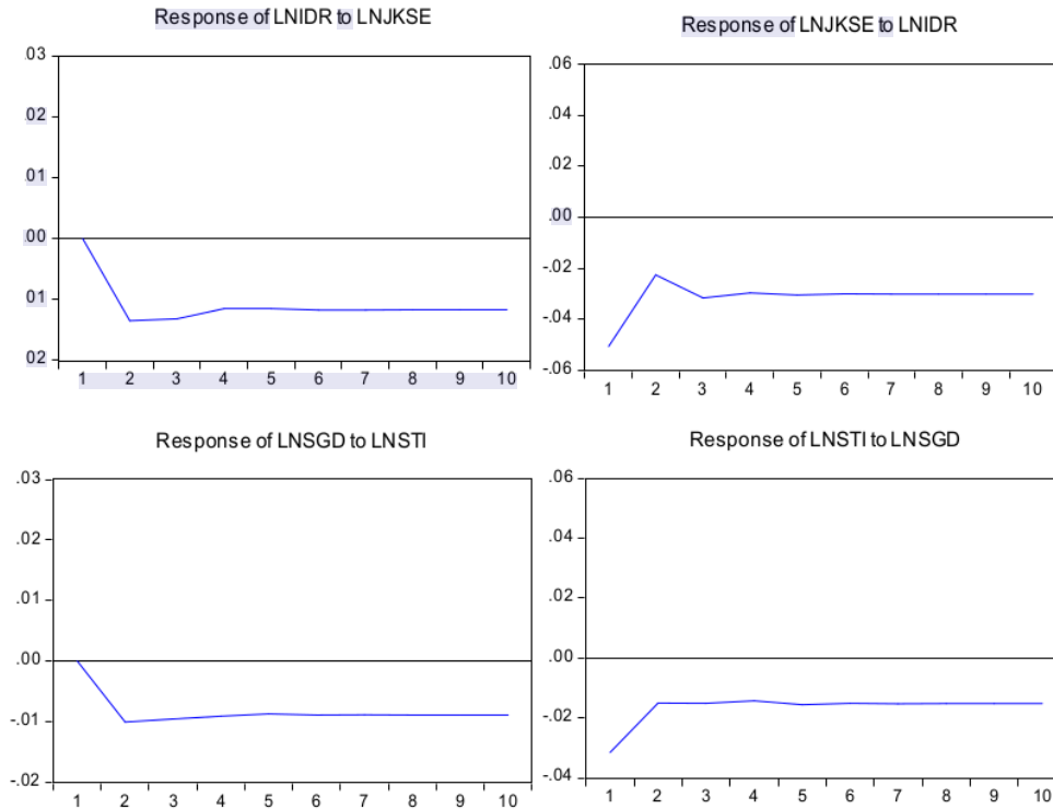
Figure 2: Results of the Impulse Response Function
