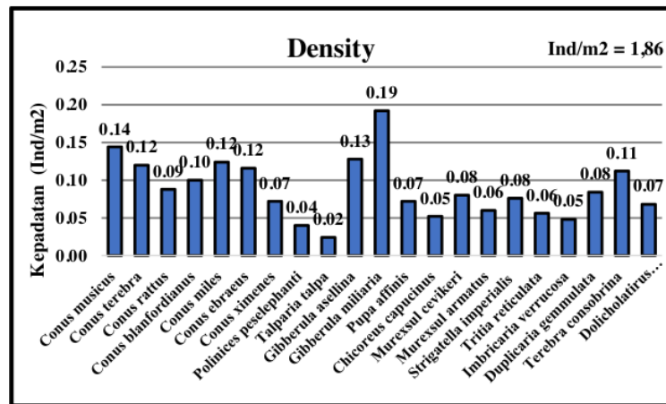
Figure 6. Mollusca Density Diagram in the Subtidal Zone
