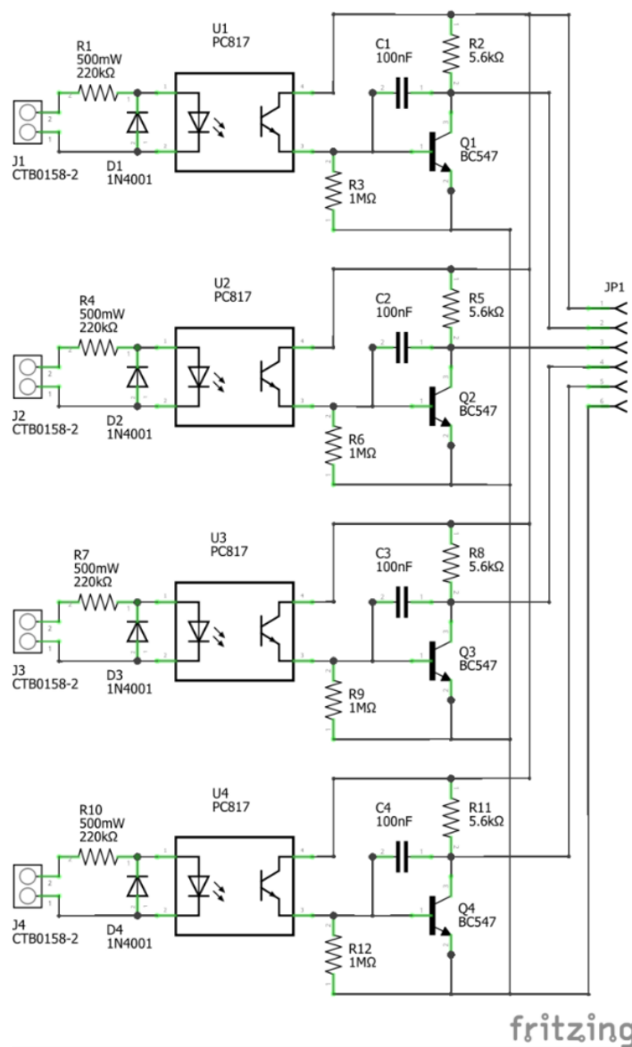
Gambar 3. Skematik 220 VAC line interface
