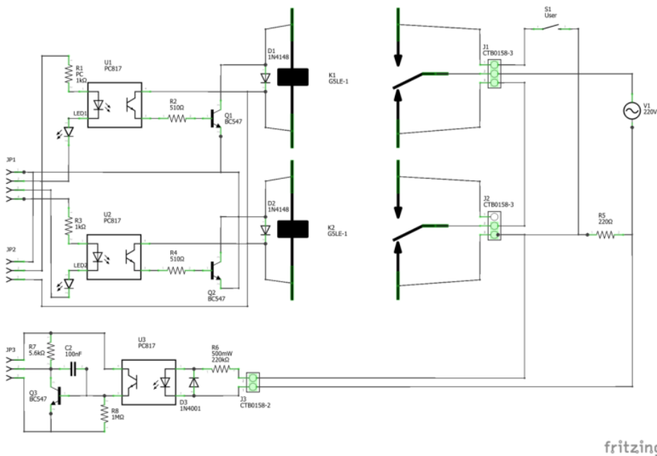
Gambar 4. Rangkaian logic switch, user switch, penerangan dan monitor tegangan
