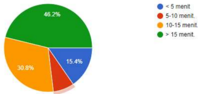
Figure 9. Task Duration
