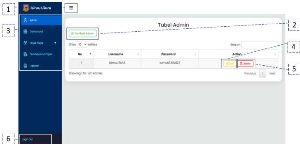
Gambar 5 Halaman administrator
