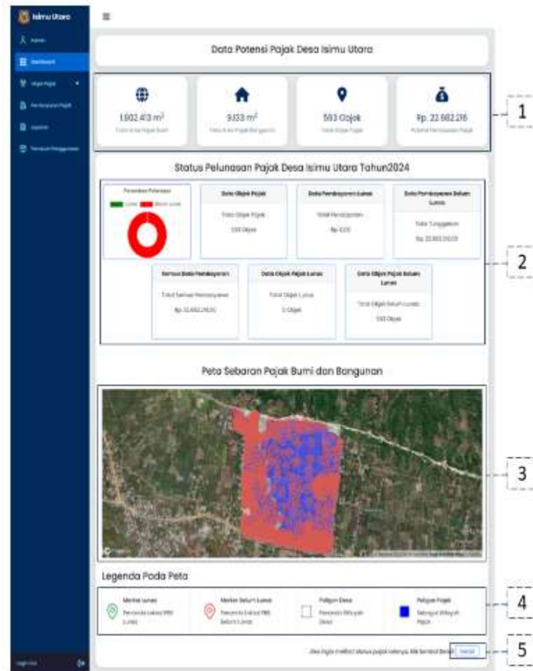
Gambar 7 Halaman dashboard
