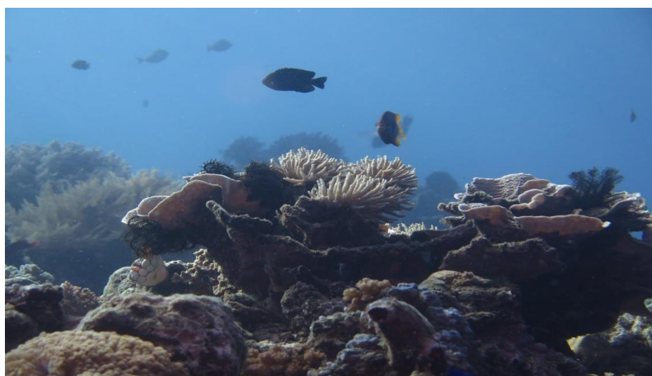
Figure 2. Condition of coral reefs at station 1.
