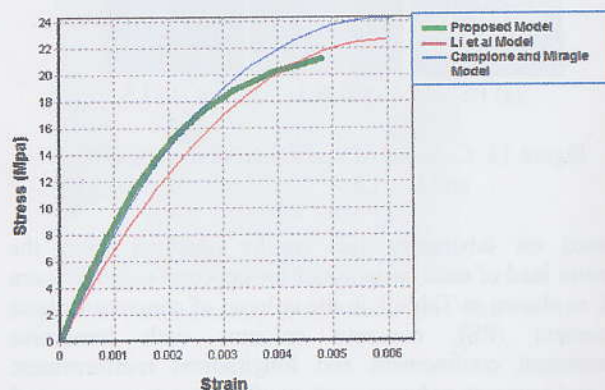
Figure 15. Proposed Model of Confined Stress Strain Curve with Li et al, and Campione and Miragle Model
