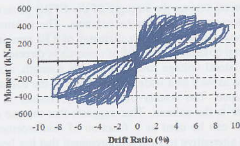
Figure 3. Column BR-C8-1, retrofitted with 4 plies of CFRP sheets
