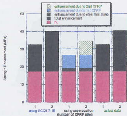
Figure 11. Strength Enhancement using Li and Fang 2004 Data (D=300mm, d=250mm, L=600mm, p_s = 1.41\% , p_{cc}=0.76\% , f_{yh}=274.7\text{Mpa} , t=0.11\text{mm} , f_{yfrp}=4120.2\text{Mpa} , f_c'=17.2\text{Mpa} )
