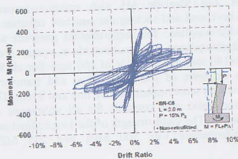
Figure 2. Reference column (non-retrofitted) BR-C8,
