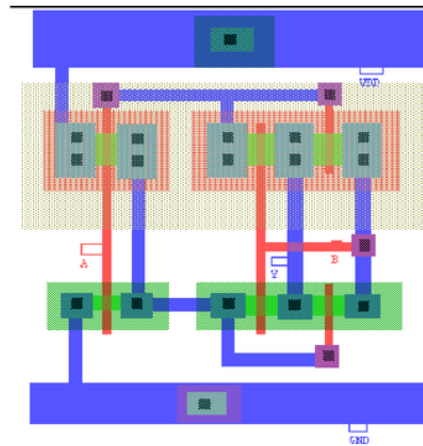
Figure 2. Layout of Basic Cell XOR 2 input
