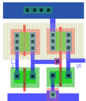
Figure 7. 1-bit shift register circuit layout
