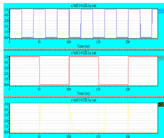
Figure 8. Spice simulation of SR-1
