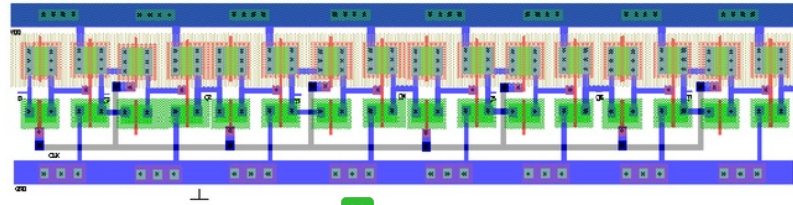
Figure 9. 8 bit shift register layout
