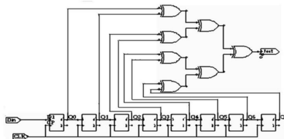
Figure 1. 8 bit parity generator circuit
