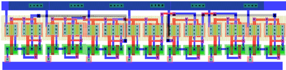
Figure 4. Layout of parity check
