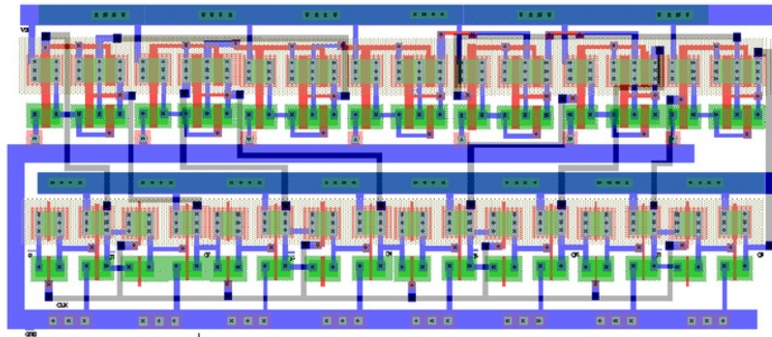
Figure 10. Complete layout of 8 bit parity generator
