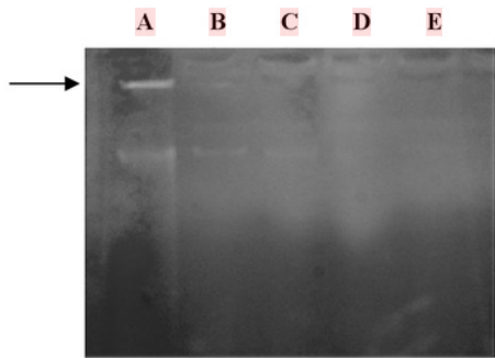
Figure 5. DNA profile of actinomycetes genome from the sediments of mangrove plants in Torosiaje, Gorontalo. A. Isolate B-1; B. Isolate C-1; C. Isolate C-2; D. Isolate X-1; E. isolate X-2. The arrow is pointing the position of DNA ribbon of actinomycetes genome
