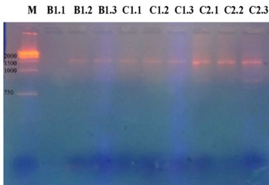
Figure 6. Profile of 16S rRNA gene from PCR in electrophoresis agarose gel with ethidium bromide as a fluorescent tag. M. Marker; B1-1 to B1-3. Isolate B-1; C1-1 to C1-3. Isolate C-1; C2-1 to C2-3. isolate C-2; The Arrow is pointing the position of DNA ribbon of actinomycetes genome
