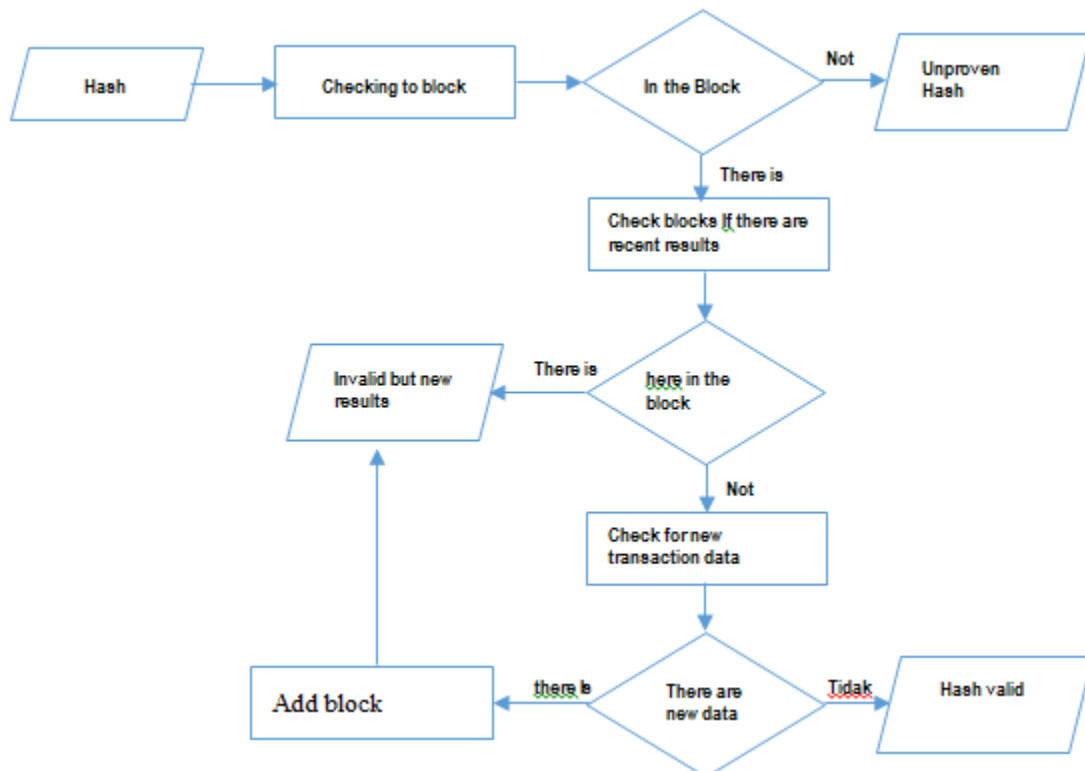
Fig. 3: Hash Proof algorithm
