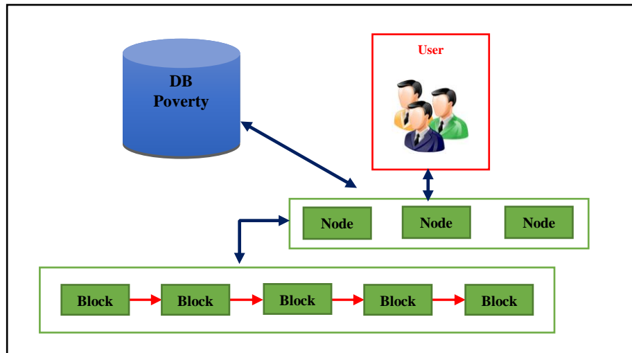
Fig 1: Poverty Data Retrieval Service Architecture
