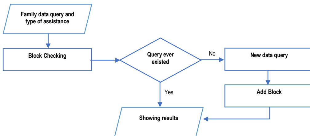
Fig 2: Data Request Algorithm
