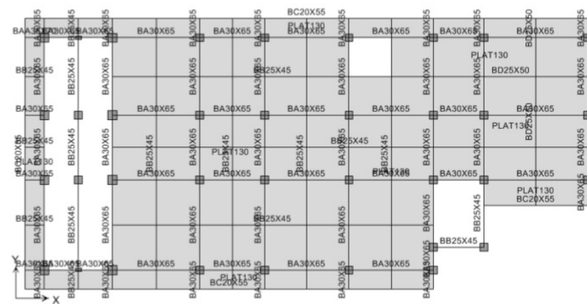
Figure 4. The 4 th floor Model
