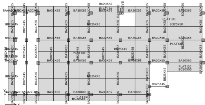
Figure 6. The 6 th floor Model
