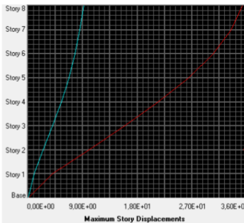
Figure 13. Displacement Due to Earthquake Load Direction Y
