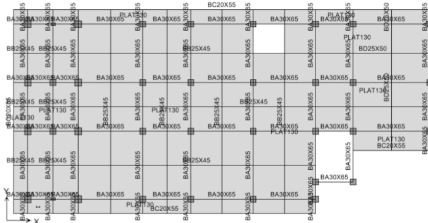
Figure 1. The 1 st floor Model
