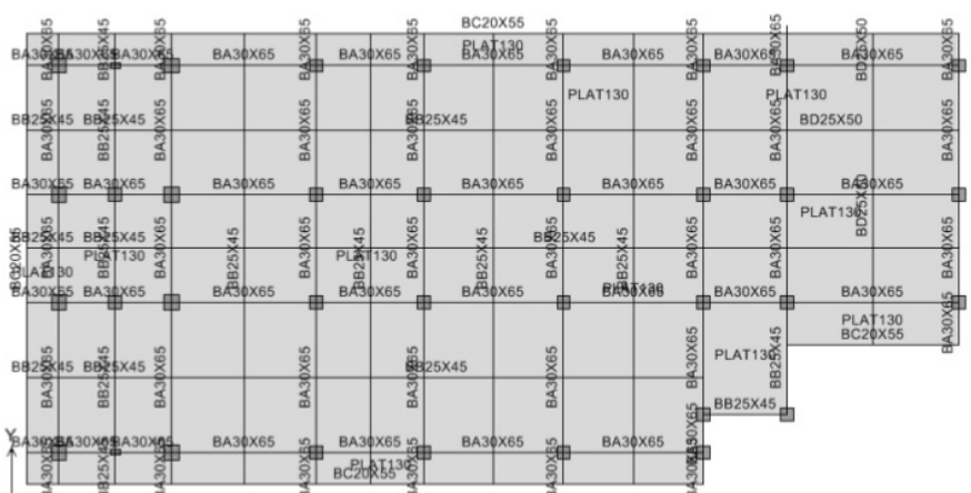
Figure 8. The 8 th floor Model
