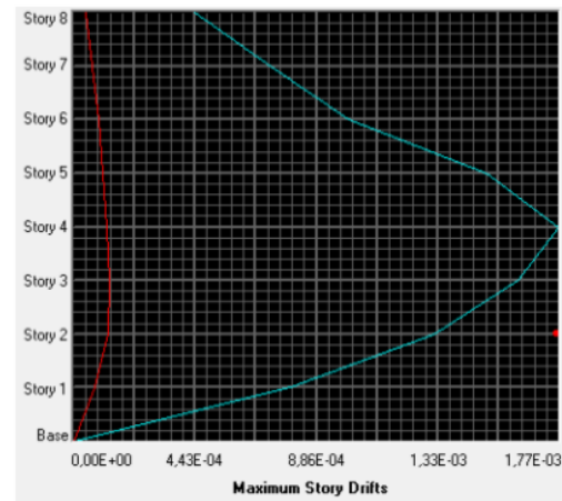
Figure 14. Story Drift Due to Earthquake Load Direction X
