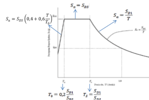
Figure 10. Spectrum Response of SNI 1726: 2012
