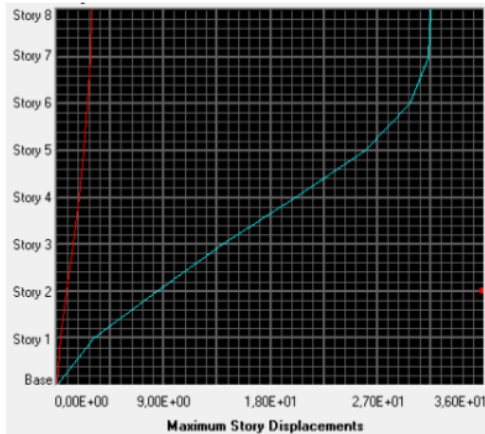
Figure 12. Displacement Due to Earthquake Load Direction X
