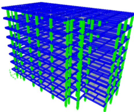
Figure 9. Modeling Results of 3 Dimensional
