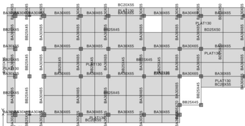
Figure 7. The 7 th floor Model
