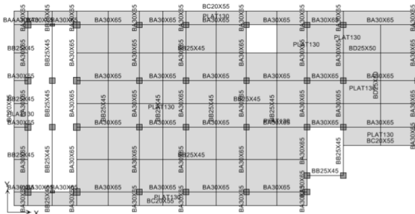
Figure 2. The 2 nd floor Model
