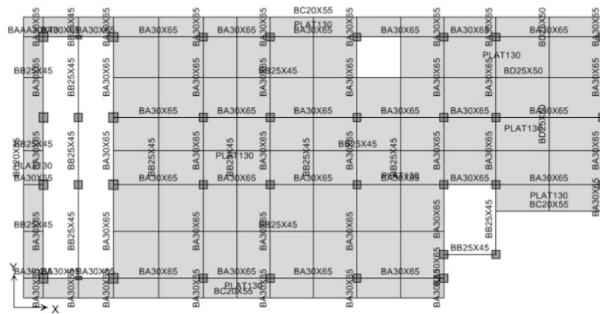
Figure 3. The 3 rd floor Model
