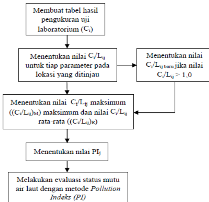
Gambar 2. Alur Perhitungan Metode Indeks Pencemaran
