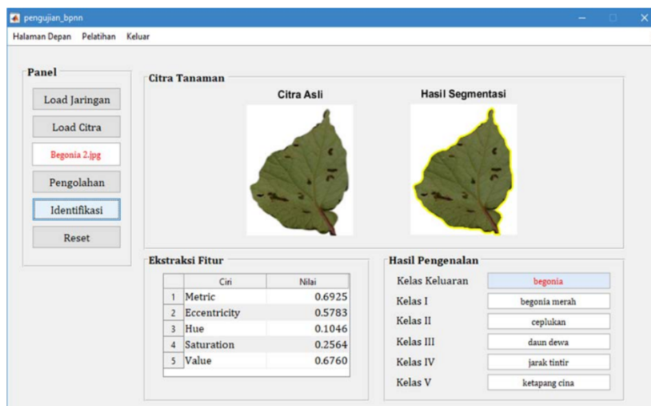
Fig. 7 Network testing process.
