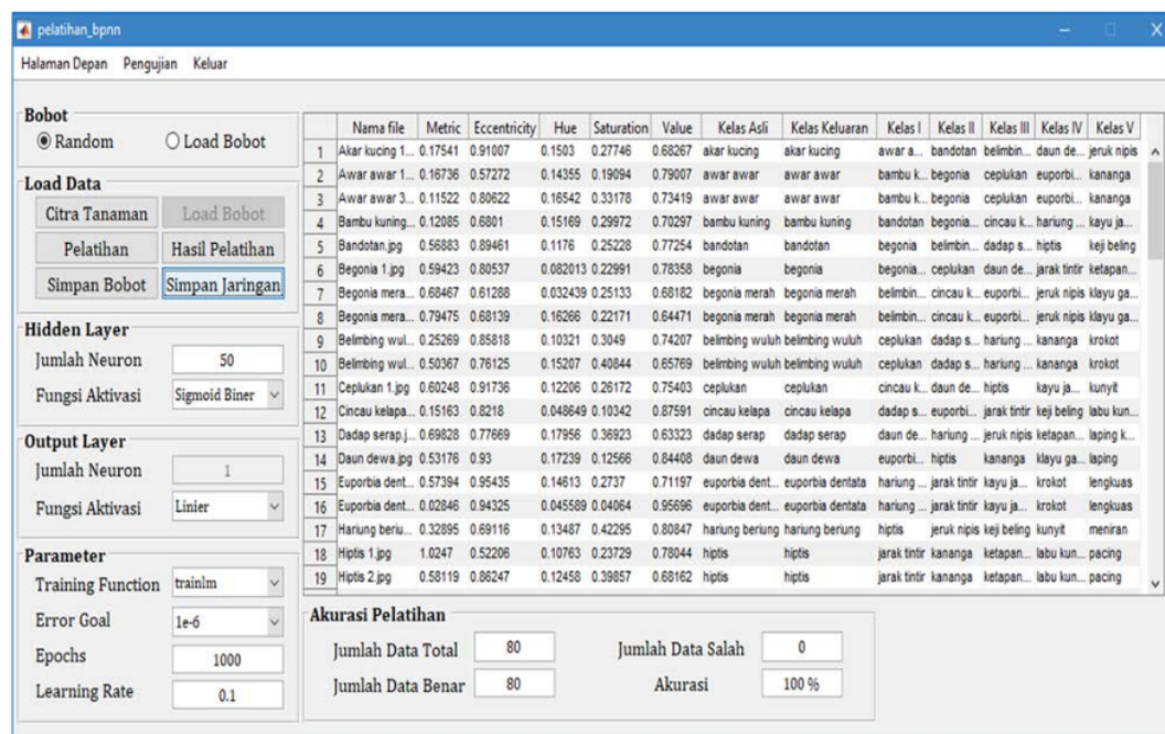
Fig. 6 Network training process.
