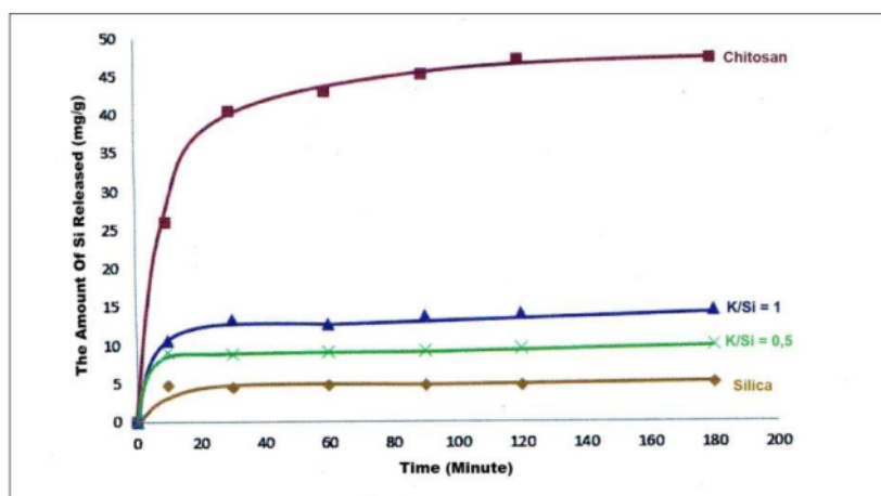
Figure 3b. Release of Si on a composite prepared with a silica mass variation in a solution of citric acid of 0.05 M
