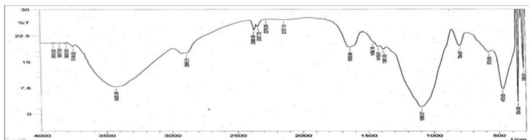
Figure 2b. Synthesis of Nanosilika-chitosan composite ratio with FTIR of 1: 0.5
