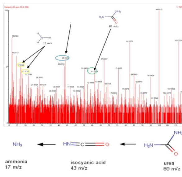
Fig 2:- Mass spectrum of urea content.
