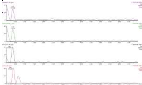
Figure 1. Chromatogram result of the control, sample A, B, and C
