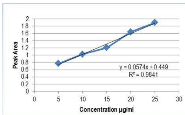
Figure 3. Analysis of calibration curve
