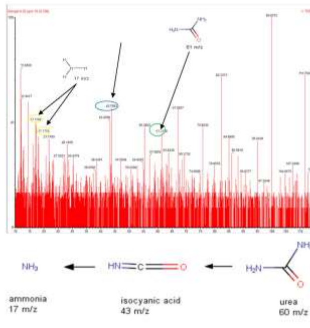
Figure 2. Mass spectrum of urea content
