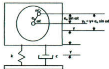
Gambar 4. Model Harmonis Teredam
