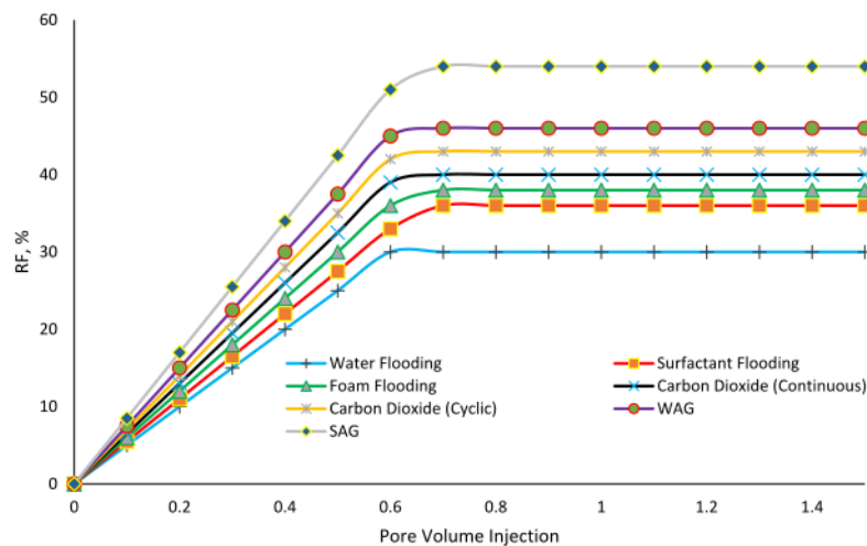
Fig. 5. Oil recovery factor for different injectivity scenarios.
