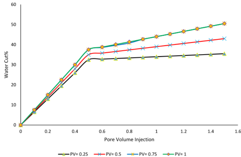
Fig. 4. Oil recovery factor in the presence of different total surfactant injection volume.
