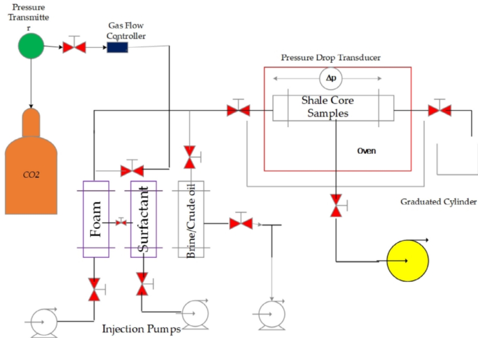
Fig. 1. Schematic of coreflooding apparatus.
