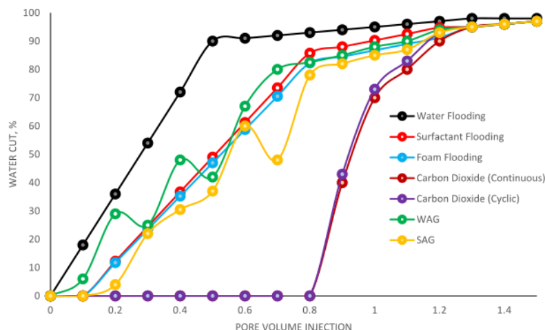
Fig. 6. Water cut for different injectivity scenarios.
