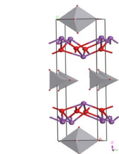
Fig 2. The one possibility of a structure that has V - O tetrahedral environment with oxygen vacancy in the equatorial site
