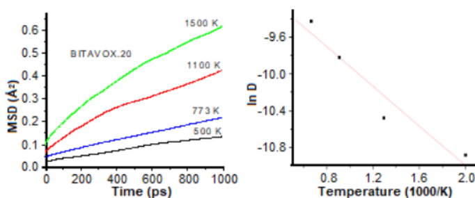
Fig 10. Oxide ion MSD and \ln D vs. 1/T plot of \text{Bi}_2\text{Ta}_{0.2}\text{V}_{0.8}\text{O}_{5.5}
