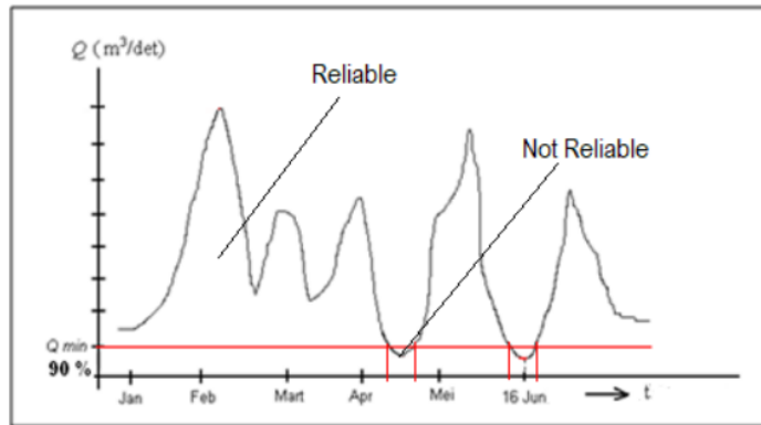
Figure 2. Determination of 90% main discharge
