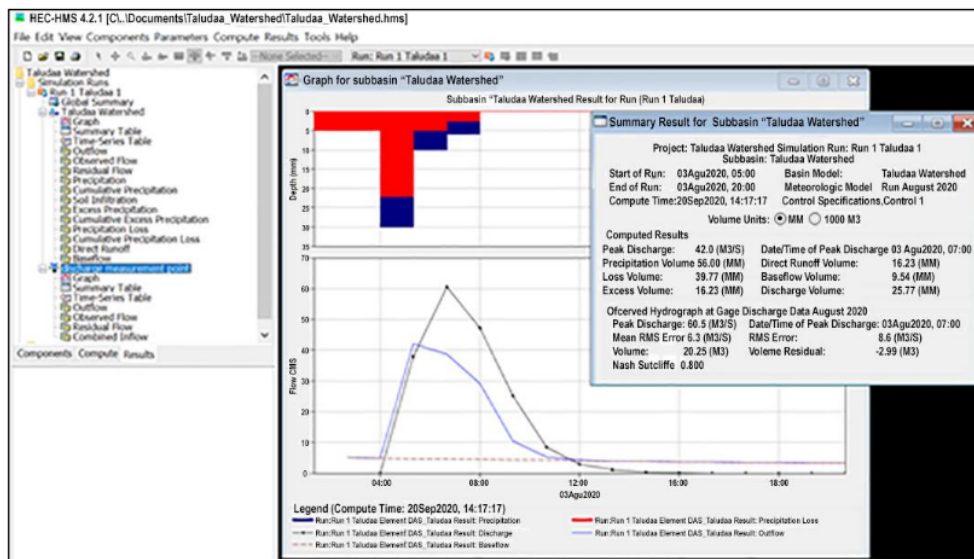
Figure 7. The results of modeled rain into discharge using HEC-HMS
