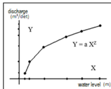
Figure 1. The curve of water level versus discharge
