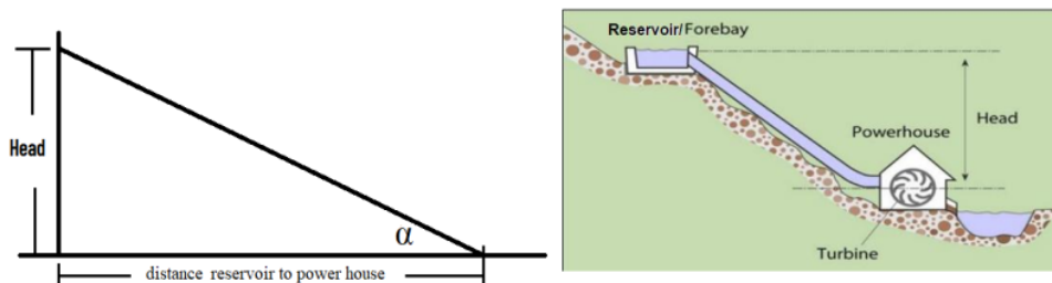
Figure 3. Determination of the head based on distance from the reservoir to the powerhouse
