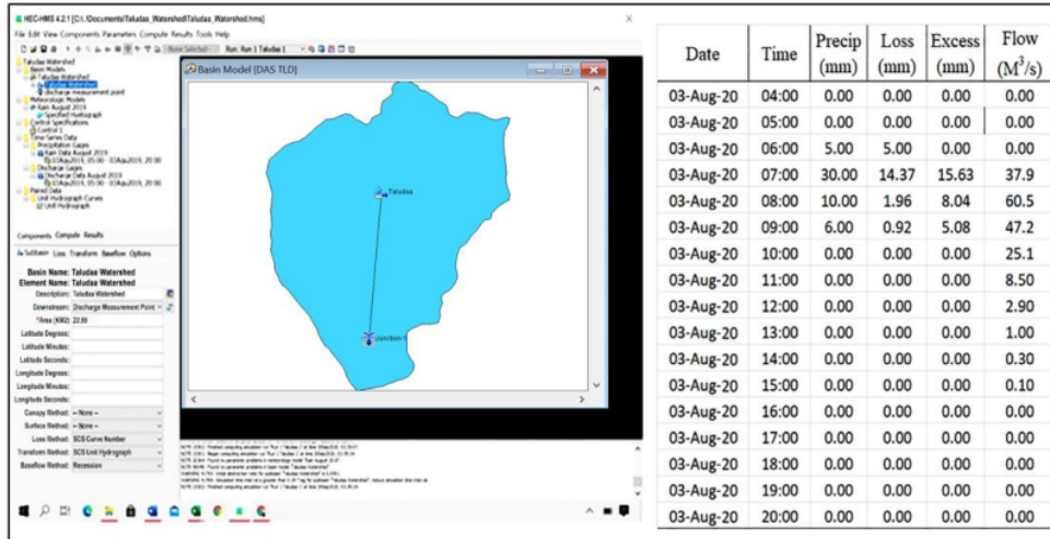
Figure 6. HEC-HMS model process for determining river discharge
