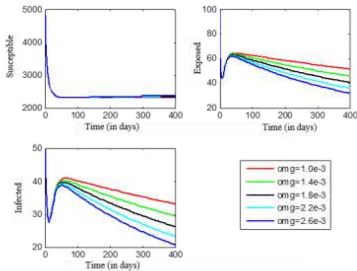
Figure 3. Mosquito population dynamics after the increase in human recovery rate ( \omega_h ) parameter value
