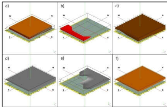
Fig.12. Lithology distribution models in the Libungo hot springs. a) Lithology model 3D; b) Lithology isopach 3D andesite; c) Lithology isopach 3D volcanic breccia; d) Lithology isopach 3D silty clay; e) Lithology isopach 3D clay; and f) Lithology isopach 3D soil.
