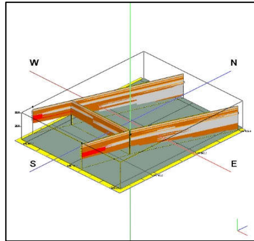
Fig 11. Litologi fence that shows lithology distribution of GF1 - GF6.
