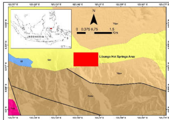
Fig.1. Regional geology of research location (Apandi and Bachri, 1997).
