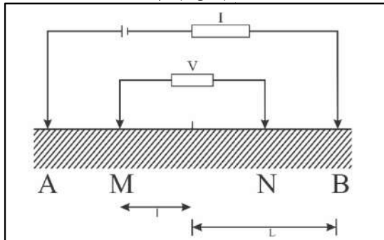
Fig. 3. Schlumberger electrode configuration (Adapted from Santoso, 2002).
