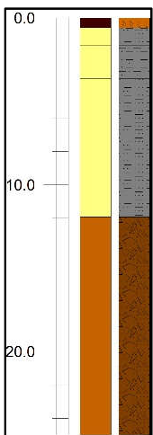
Fig 6. Single log GF2.
