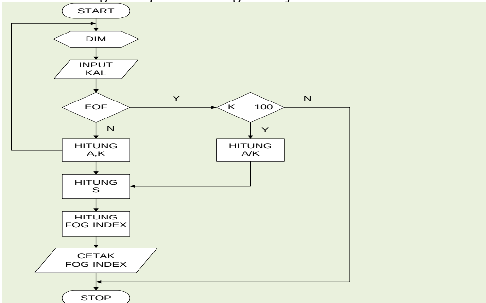
Gambar 2.1 Flowchart Fog Indeks (Robert Gunning).
