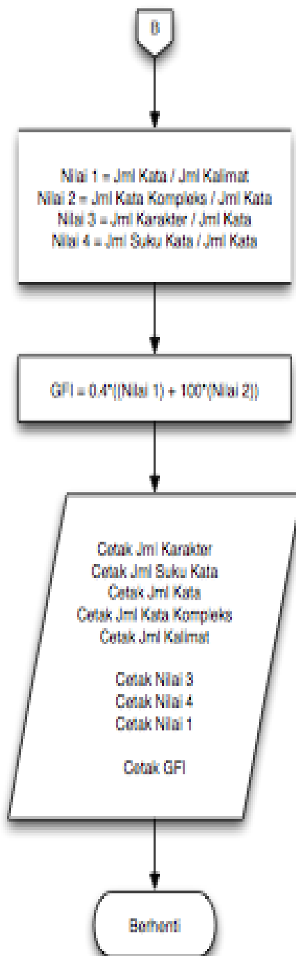
Gambar 3: Lanjutan Flowchart Program
