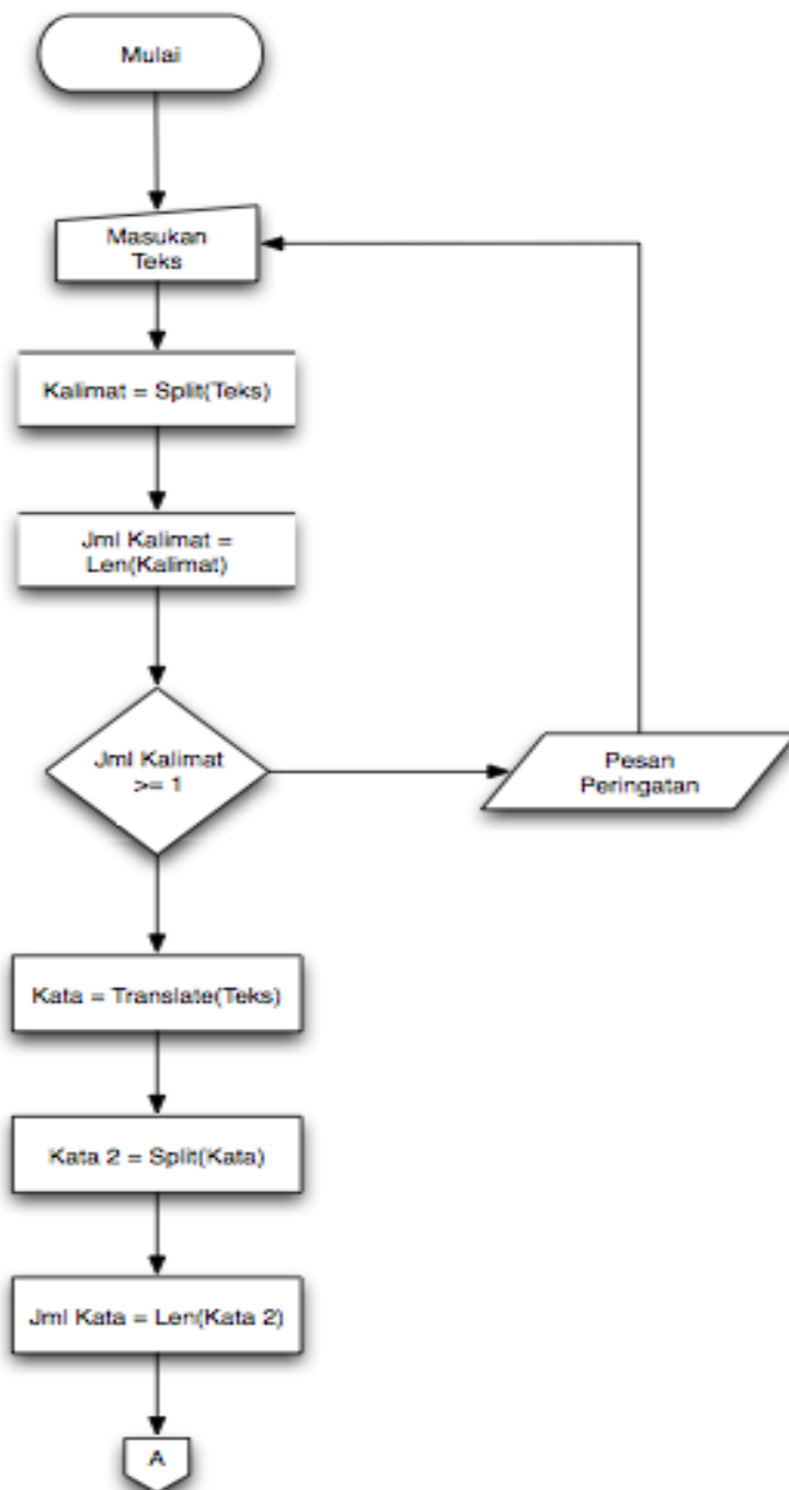
Gambar 1: Flowchart Program
