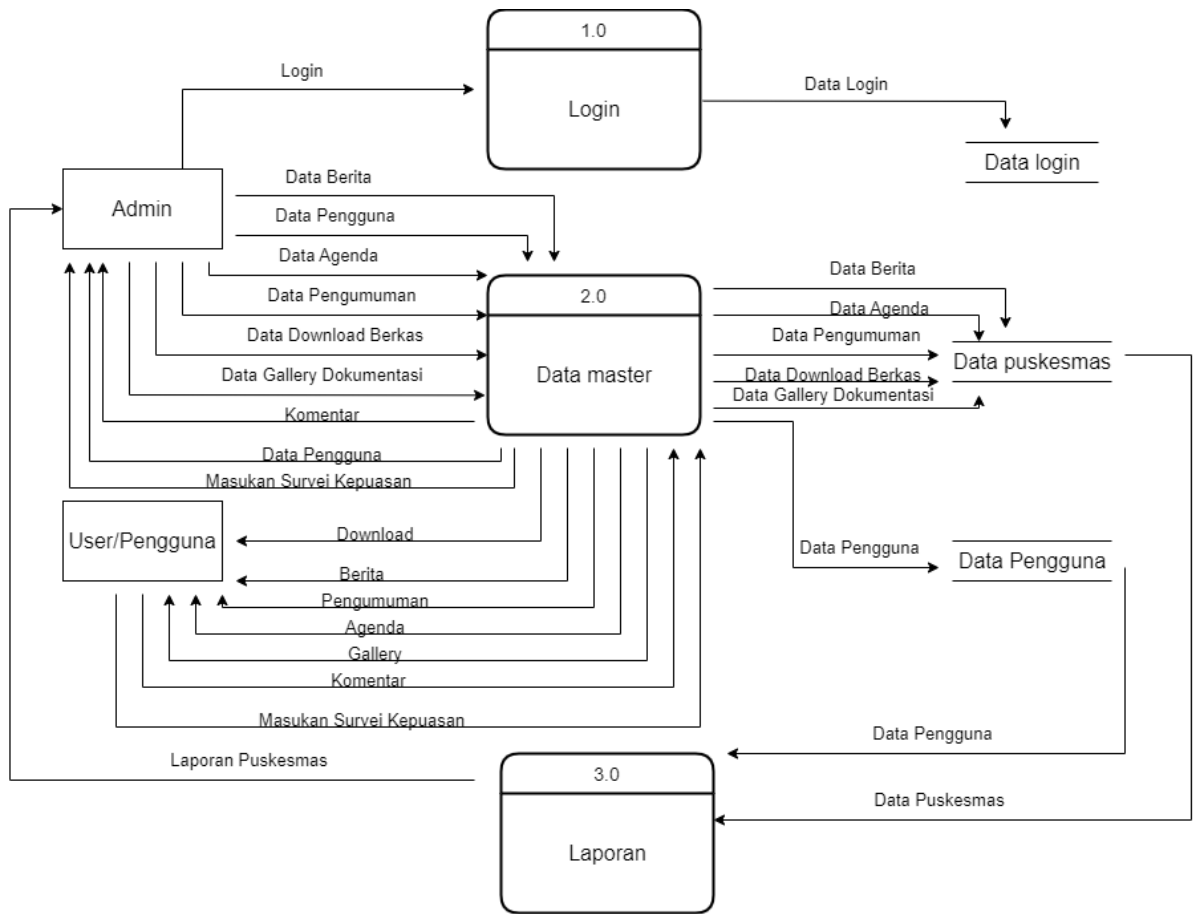
Gambar 4. 2 Data flow diagram level 1
