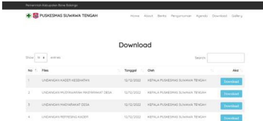
Gambar 4. 17 Tampilan Download
