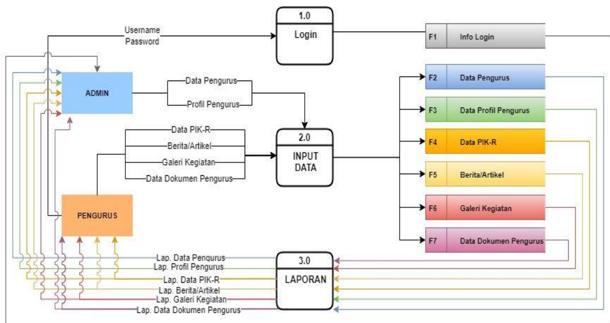
Gambar 2. DAD level 0
