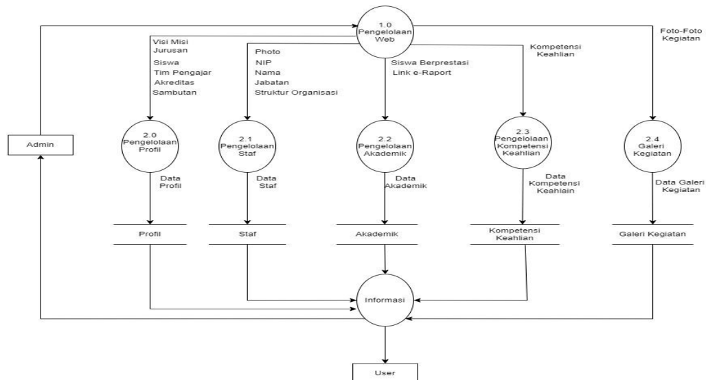
Gambar 3. DFD Level 0
